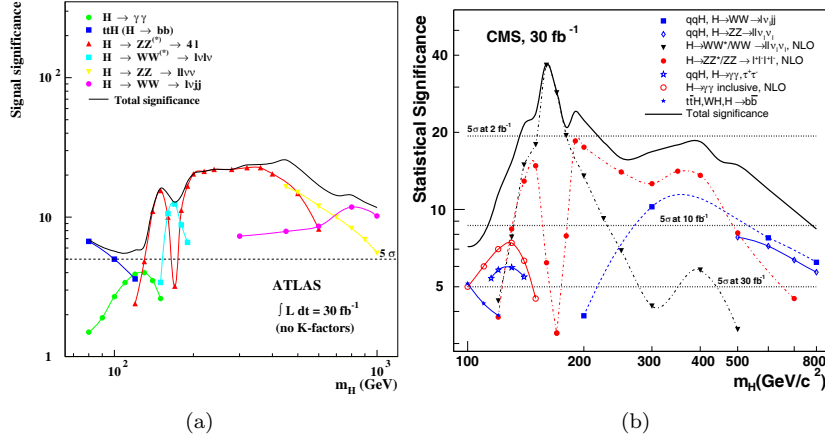
Figure 1. Expected sensitivity for the observation of the Standard Model Higgs boson signal as a function of the mass m_H with ATLAS (a) and CMS (b) with 30 \text{ fb}^{-1} integrated luminosity.
