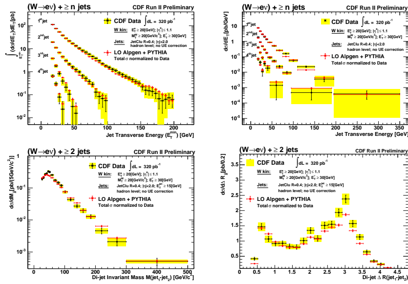
Figure 1. Top: Cumulative cross section \sigma(W \rightarrow ev + \geq n\text{-jets}; E_T^{jet}(n) > E_T^{jet}(min)) as a function of the minimum E_T^{jet}(min) (Left) and differential cross section d\sigma(W \rightarrow ev + \geq n\text{-jets})/dE_T^{jet} (Right) for the first, second, third and fourth inclusive jet sample. Bottom: Differential cross section d\sigma(W \rightarrow ev + \geq 2\text{-jets})/dM_{1j2} (Left) and d\sigma(W \rightarrow ev + \geq 2\text{-jets})/dR_{1j2} (Right) respectively as a function of the invariant mass and angular separation of the leading 2 jets. Data are compared to Alpgen+PYTHIA predictions normalized to the measured cross section in each jet multiplicity sample.
