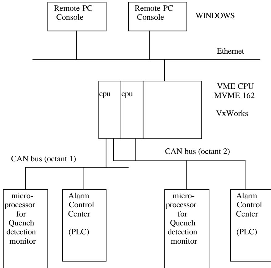
Figure 1. Schematic drawing of the hardware architecture for a quadrant
