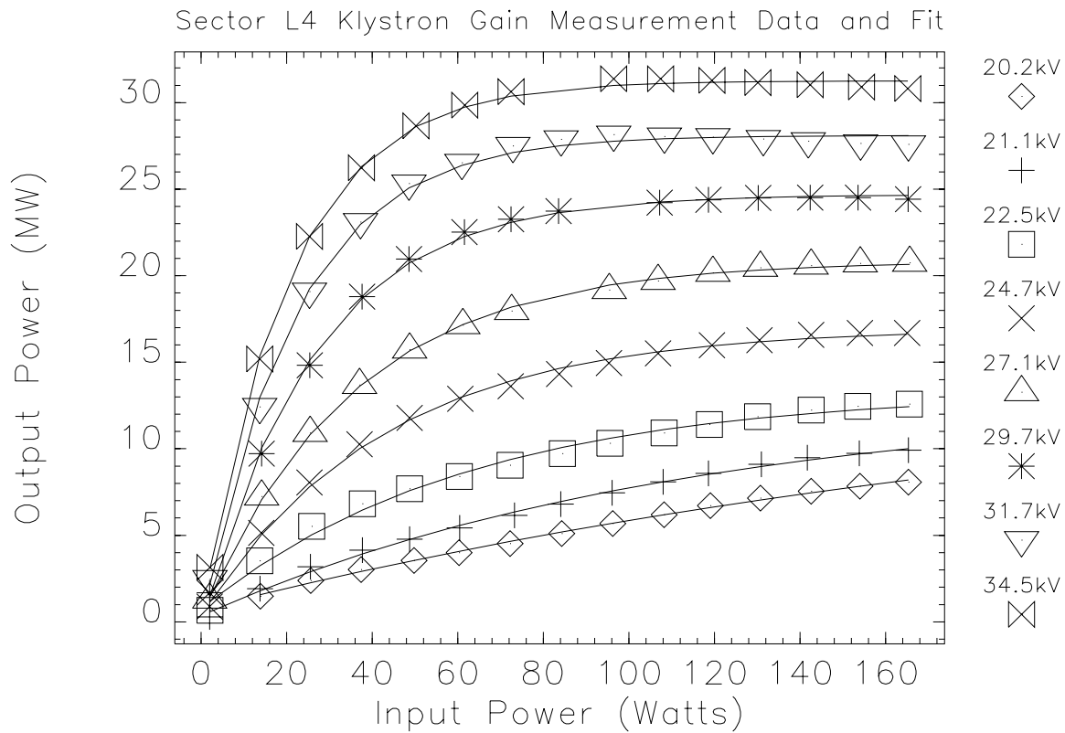
Figure 4: Measurements and fits for klystron output power vs input power for various PFN voltages.
