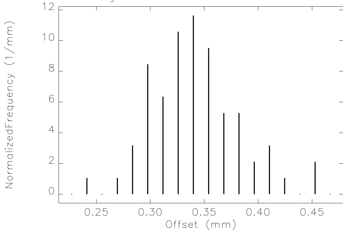
Figure 6: Histogram of particular BPM-to-quadrupole offset as estimated from numerous BPMs.
