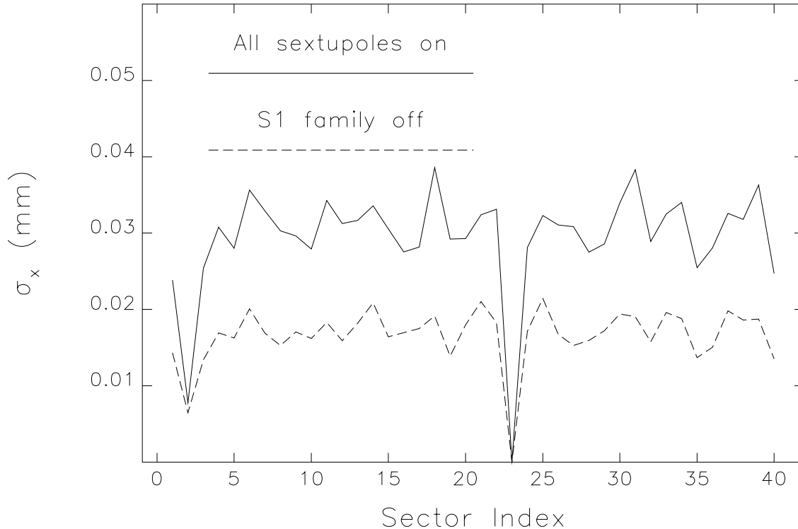
Figure 2: rms orbit motion as a function of BPM around the ring for two lattice configurations.
