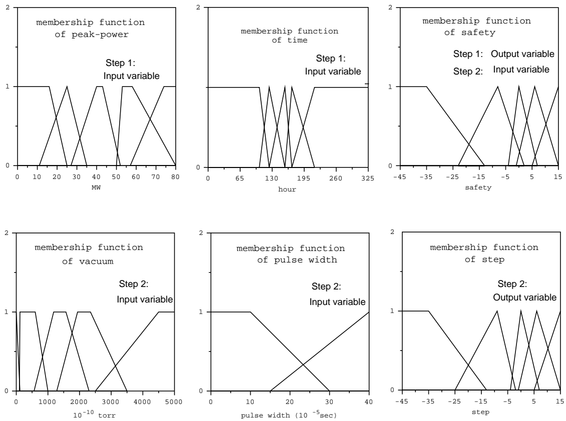
Figure. 6. Membership functions of the RF conditioning
