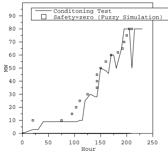
Figure. 8. Result of the step1 fuzzy inference
