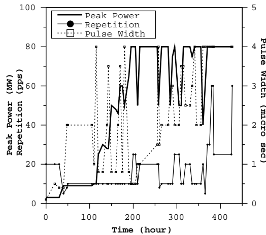
Figure. 2. Summary of the RF conditioning test
