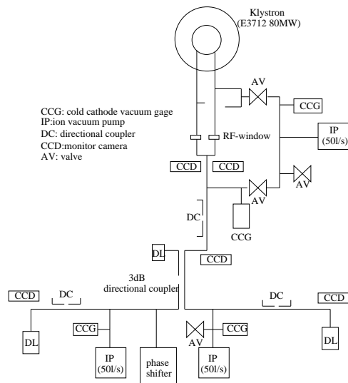
Figure. 1. High Power test bench
