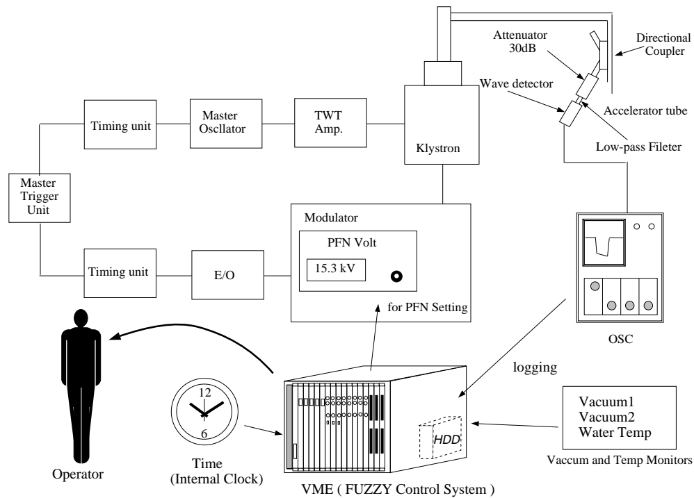
Figure. 3. Design of the conditioning system using fuzzy logic
