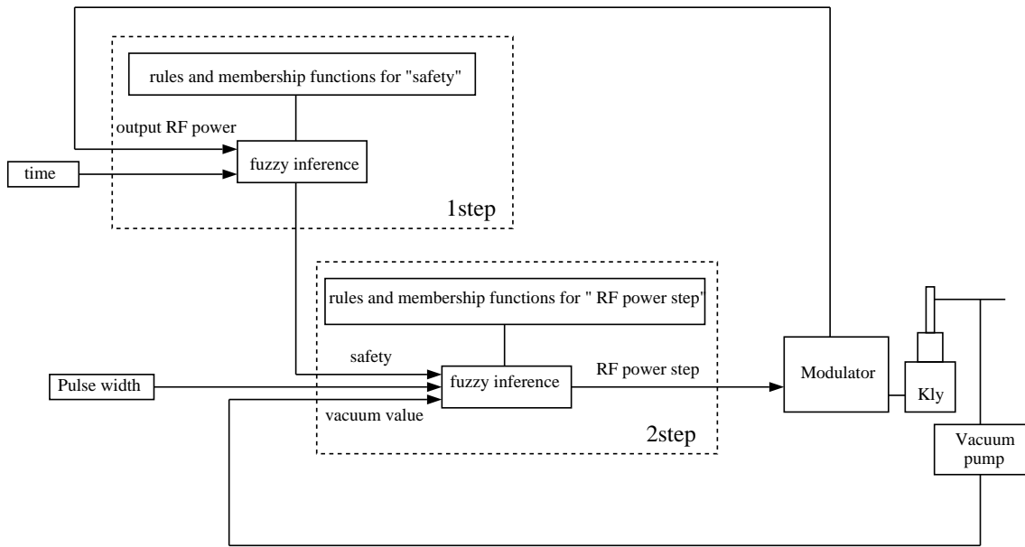
Figure. 5. Block diagram of the RF conditioning system
